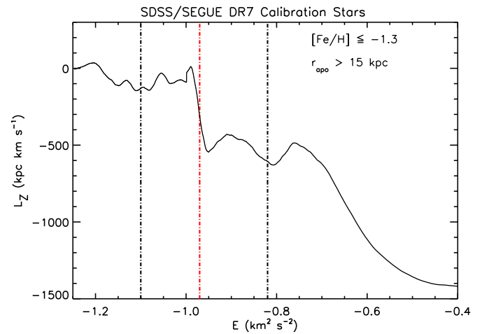
Figure 3. Mean angular momentum in the z direction as a function of the total energy (in units of 10^5 ) for the 8039 SDSS/SEGUE DR7 calibration stars with metallicity [\text{Fe}/\text{H}] \leq -1.3 and r_{\text{apo}} > 15 \text{ kpc} . A moving average with overlapping bins of 200 stars is applied. The vertical red dot-dashed line denotes the mean point of the transition zone between the inner halo and outer halo, while the vertical black dot-dashed lines represents the adopted transition zone.
