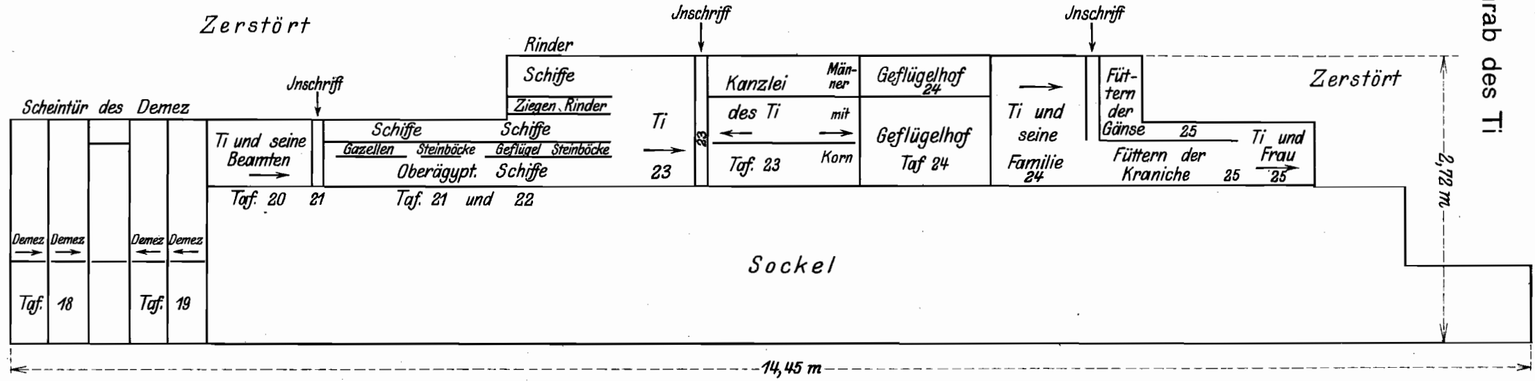
Pfeilerhof: Westwand
